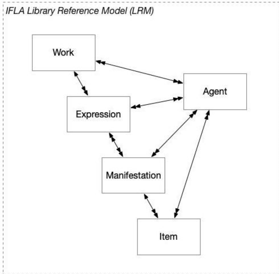
Figure 1: LRM and BIBFRAME
